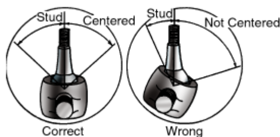
Gambar 180. Ball joint.
