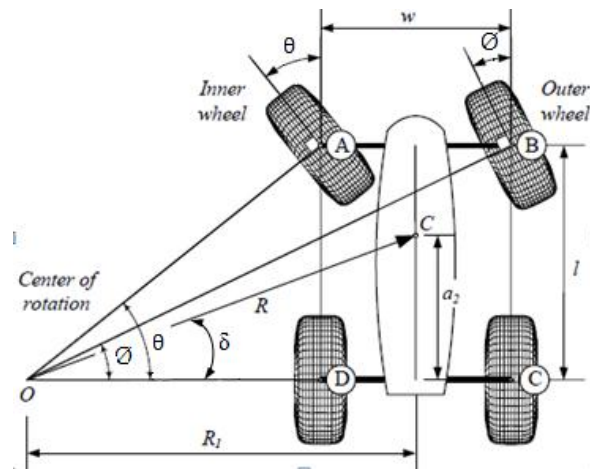
Gambar 150. Prinsip ankerman
