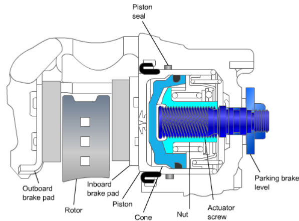
Gambar 53. Rem parkir tipe Screw-and-nut.
