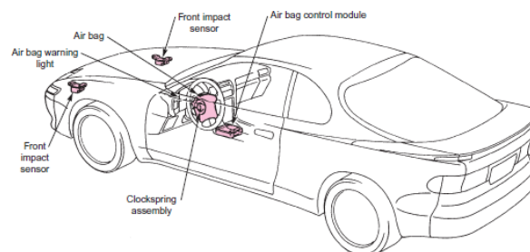
Gambar 116. Air bag system.
