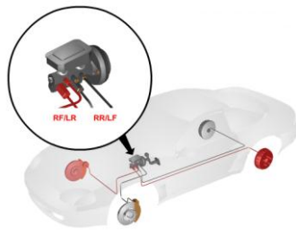
Gambar 58. Sirkuit diagonal.
