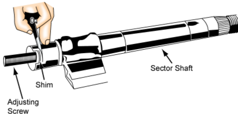
Gambar 172. Poros sector.
