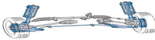
Gambar 126. Unit rak and pinion.
