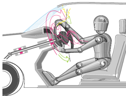
Gambar 125. Anti-theft test.
