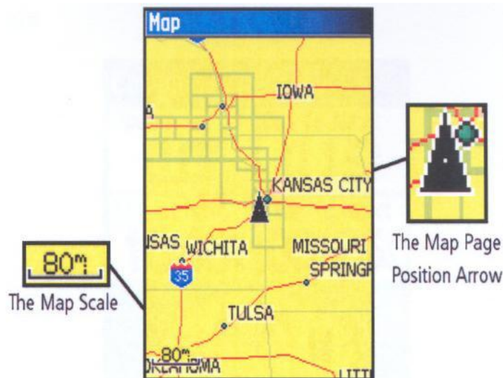
Gambar 5.6 Map page
