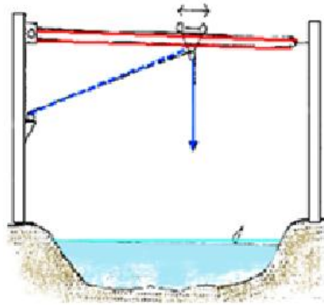
Gambar 6.9 Metode Winch cable
