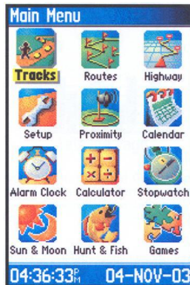
Gambar 5.9 Main menu
