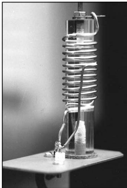
Gambar 2.3. Bagian Loading Coil antenna vertikal 5/8 \lambda
