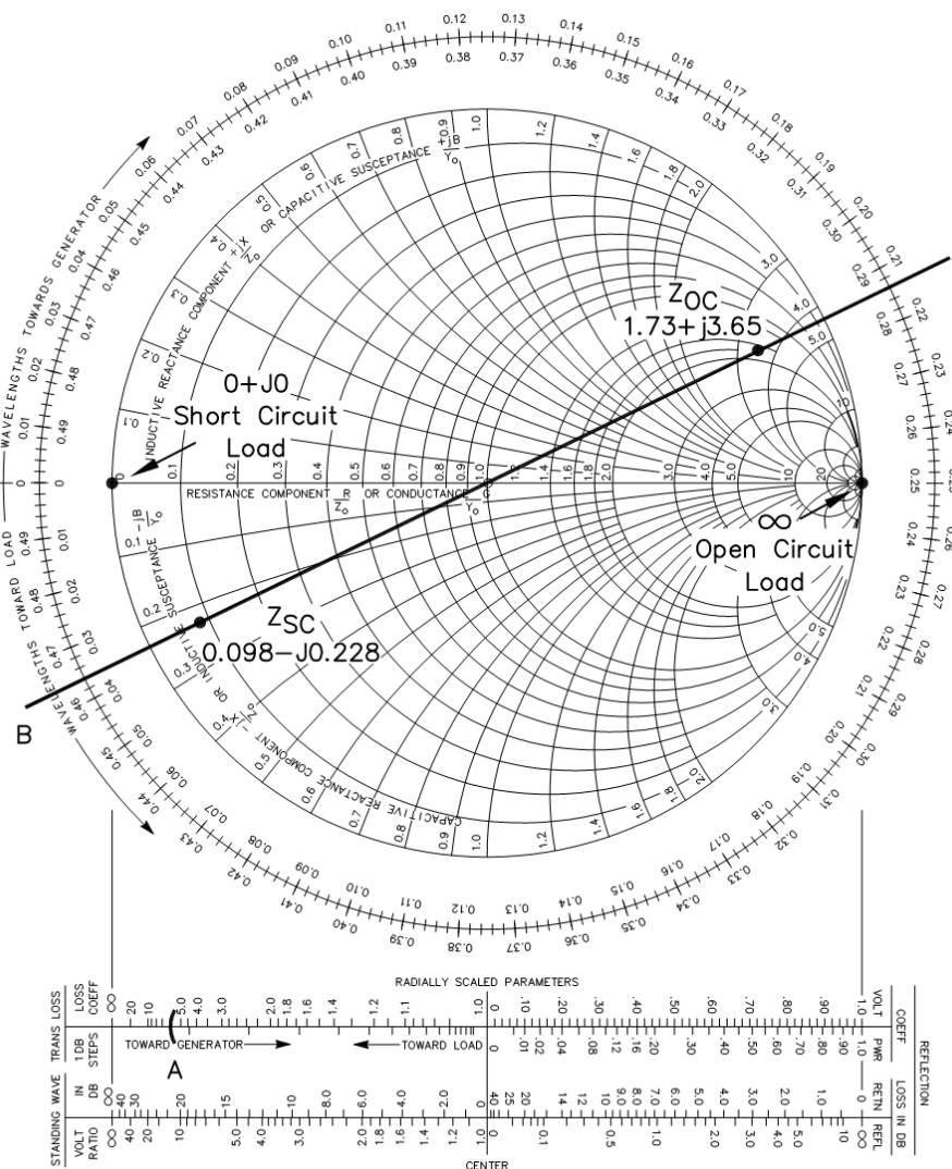
Gambar 6.7. Admittance
