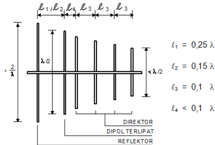
Gambar 4.18 Antena Yagi
