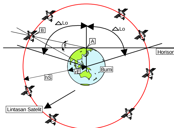
Gambar 7.10 Orbit
