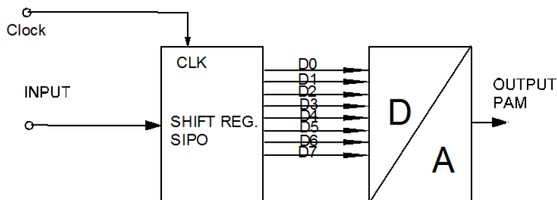
Gambar 20.4 Blok demodulator PAM
