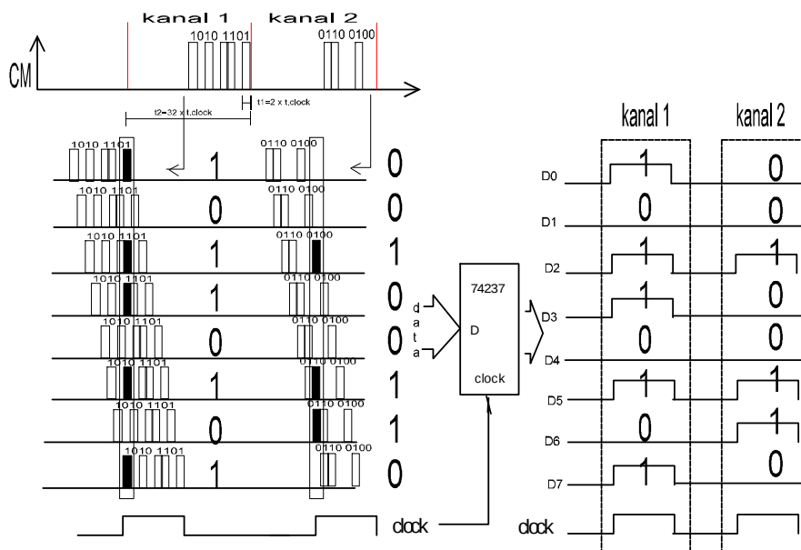
Gambar 20.3 D-Flip flop
