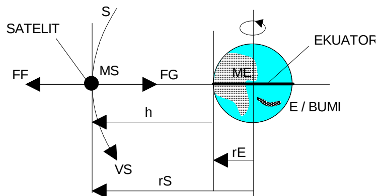
Gambar 7.5 Orbit satelit
