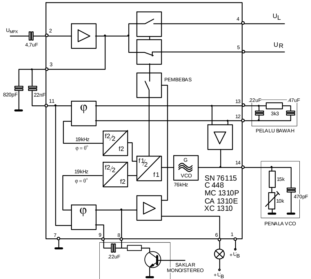
Gambar 17.20 Stereo Decoder
