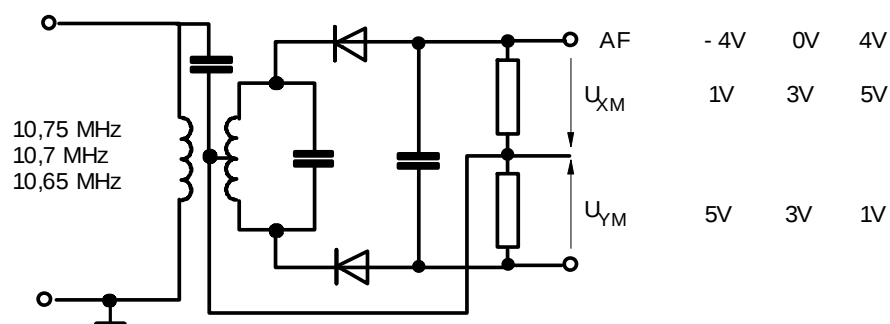
Gambar 15.10 FM demodulator
