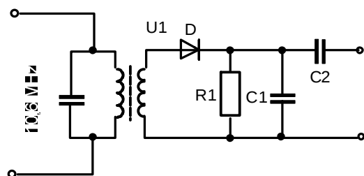
Gambar 15.6 demodulator FM
