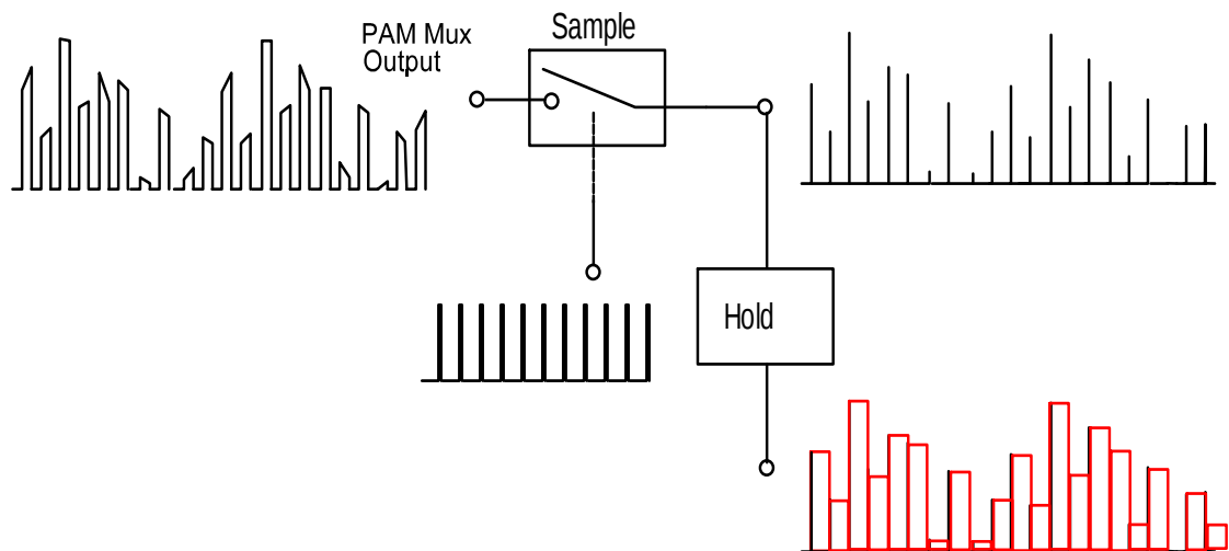
Gambar 19.8 Sample & hold
