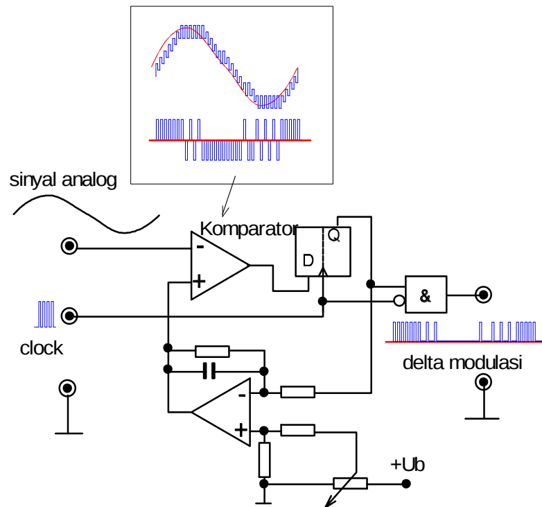
Gambar 18.1 Delta modulator
