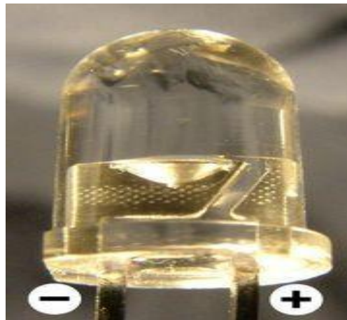
Gambar 28. LED
