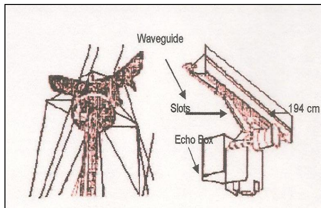
Gambar 96. Antenne Radar
