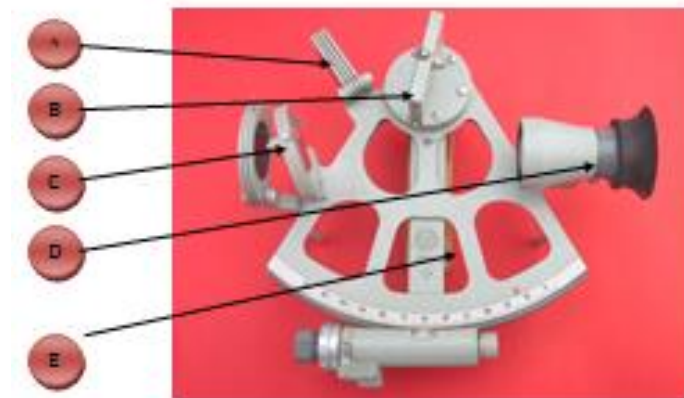
Gambar 69. Sextan
