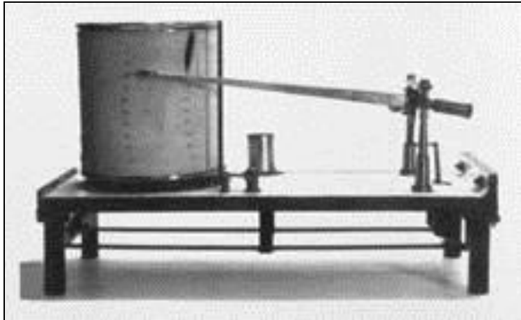
Gambar 86. Hygrometer rambut
