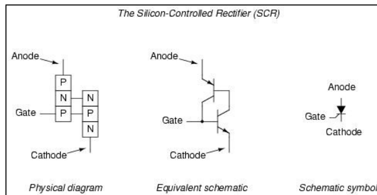
Gambar 33. Diagram Skema SCR
