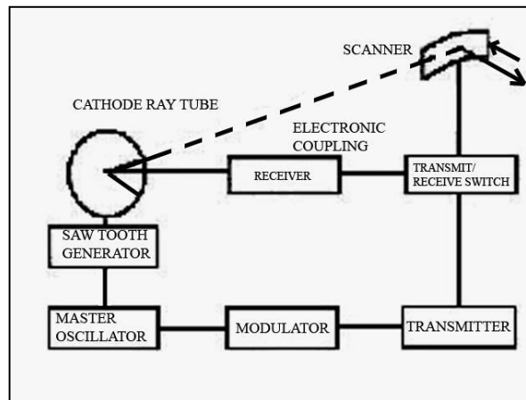
Gambar 97. Diagram Sederhana Sistem Radar
