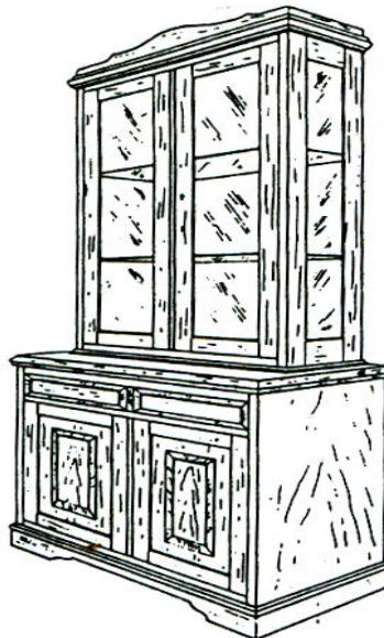
Gambar. Gambar Isometri Lemari Hias ( China Cabinet )
