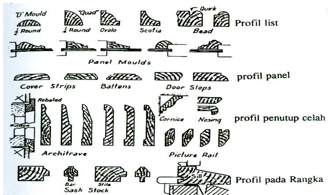
Gambar 11. Macam-macam Profil
