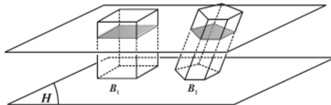
Gambar 68. Prinsip Cavalieri
