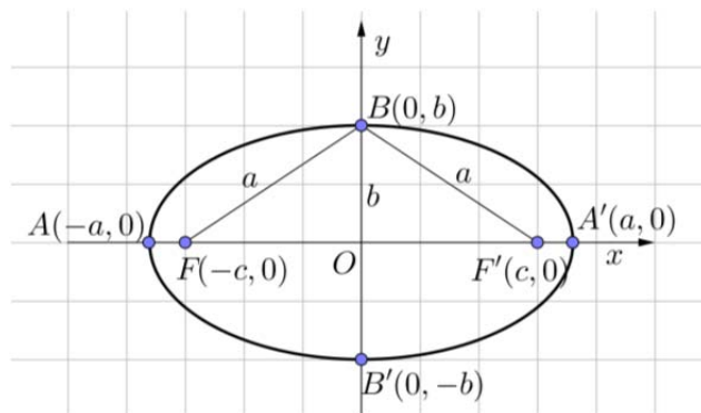
Gambar 107. Unsur-unsur ellips
