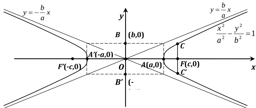
Gambar 110. Unsur-unsur hiperbola
