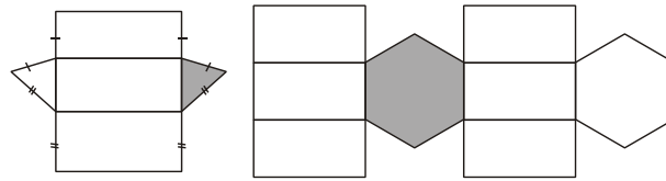
Gambar 71. Jaring-jaring Prisma
