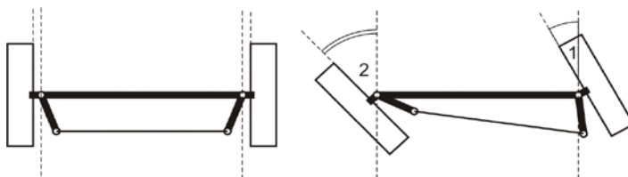
Gambar 24. Ackermann Steering Geometry
