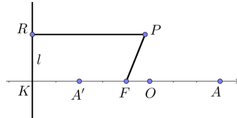
Gambar 105. Definisi ellips
