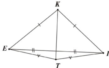
Gambar 33. Diagonal Layang-layang
