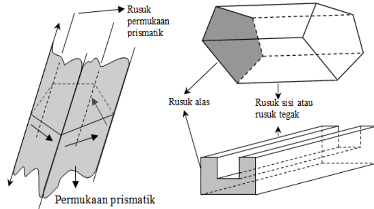
Gambar 65. Prisma
