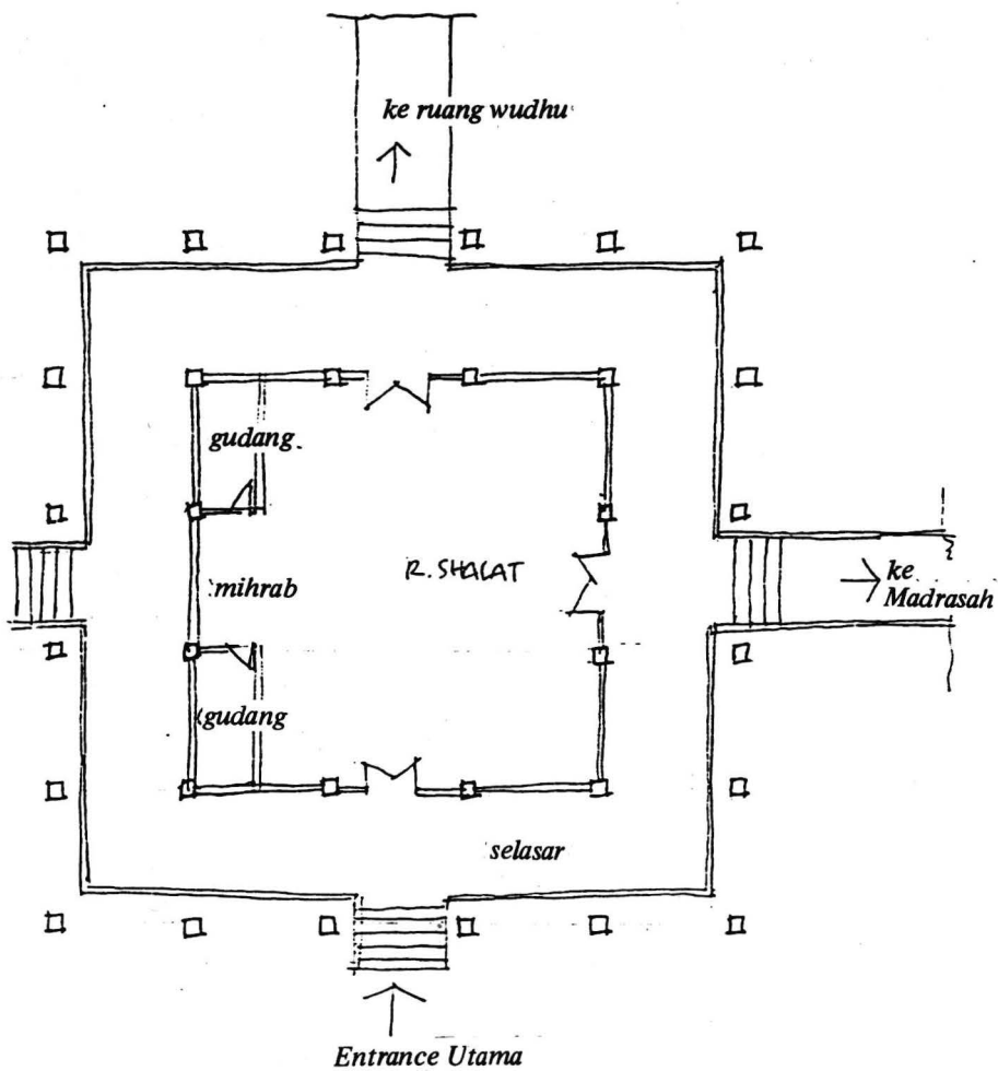
Denah Mesjid Al-Hadid.
