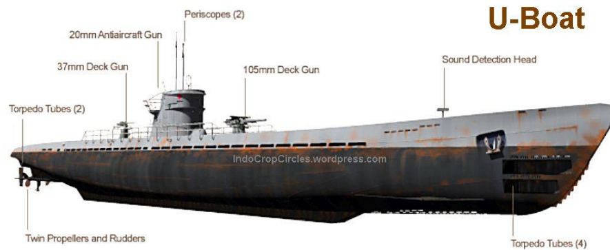
Gambar 11 Kapal Selam U-boat
