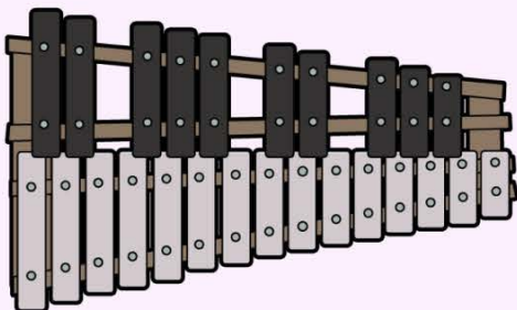
Xylophone 3621 Hertz
