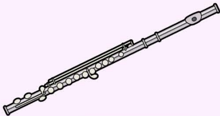
Flute 2493 Hertz
