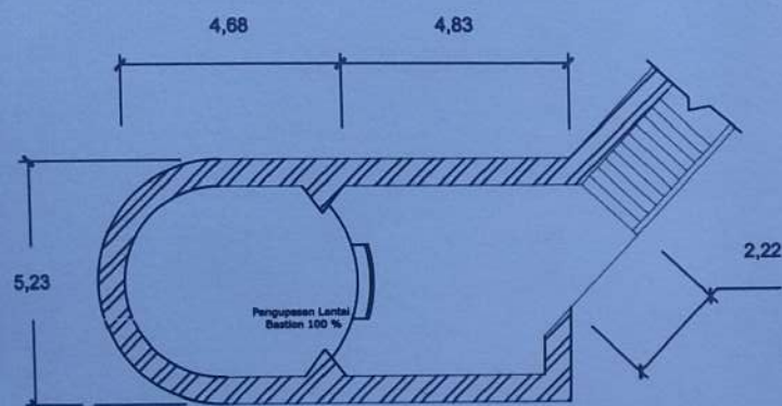
BASTION 1 BENTENG BALANG NIPA denah It 2
