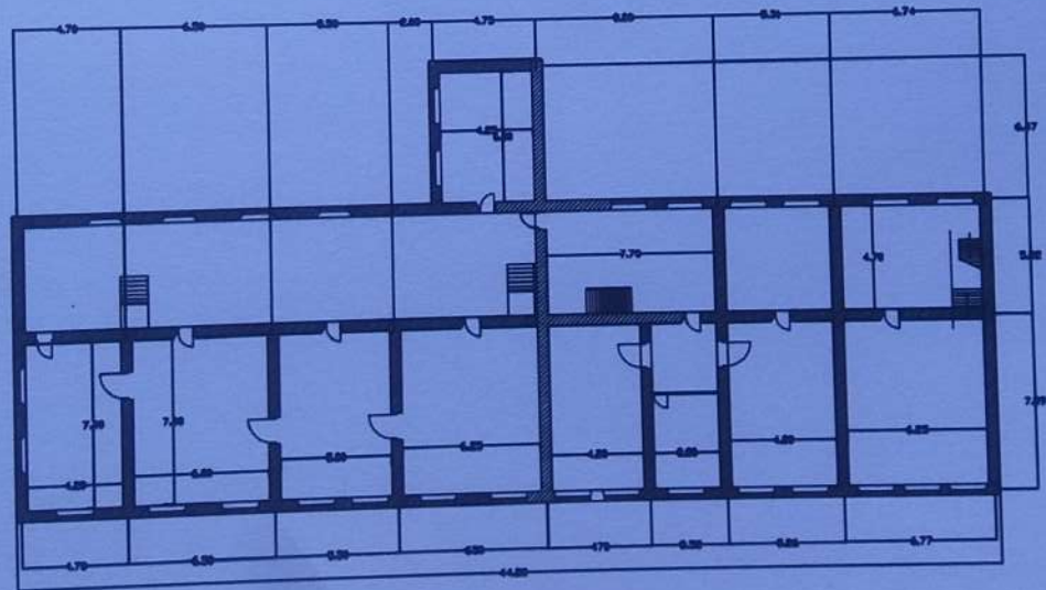
DENAH LANTAI 02 SKALA 1:200
