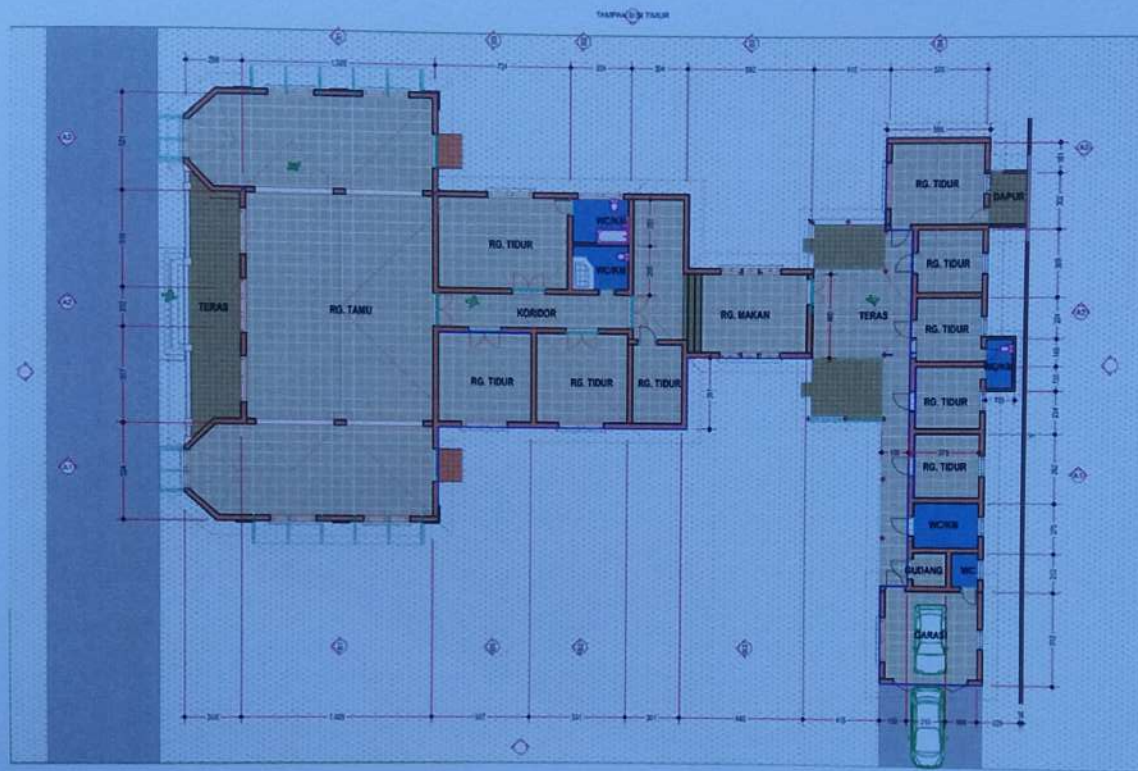
DENAH 1:200
