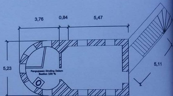
BASTION 1 BENTENG BALANG NIPA denah It 1
