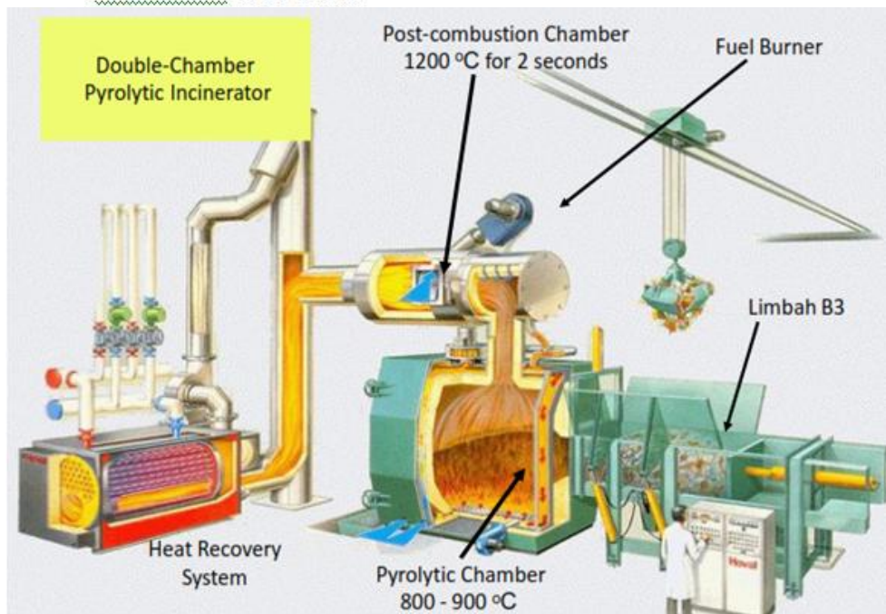
Gambar 1. Insinerator
