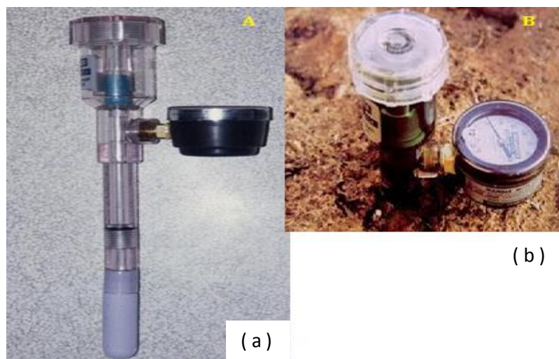
Gambar 7.1 Tensiometer
