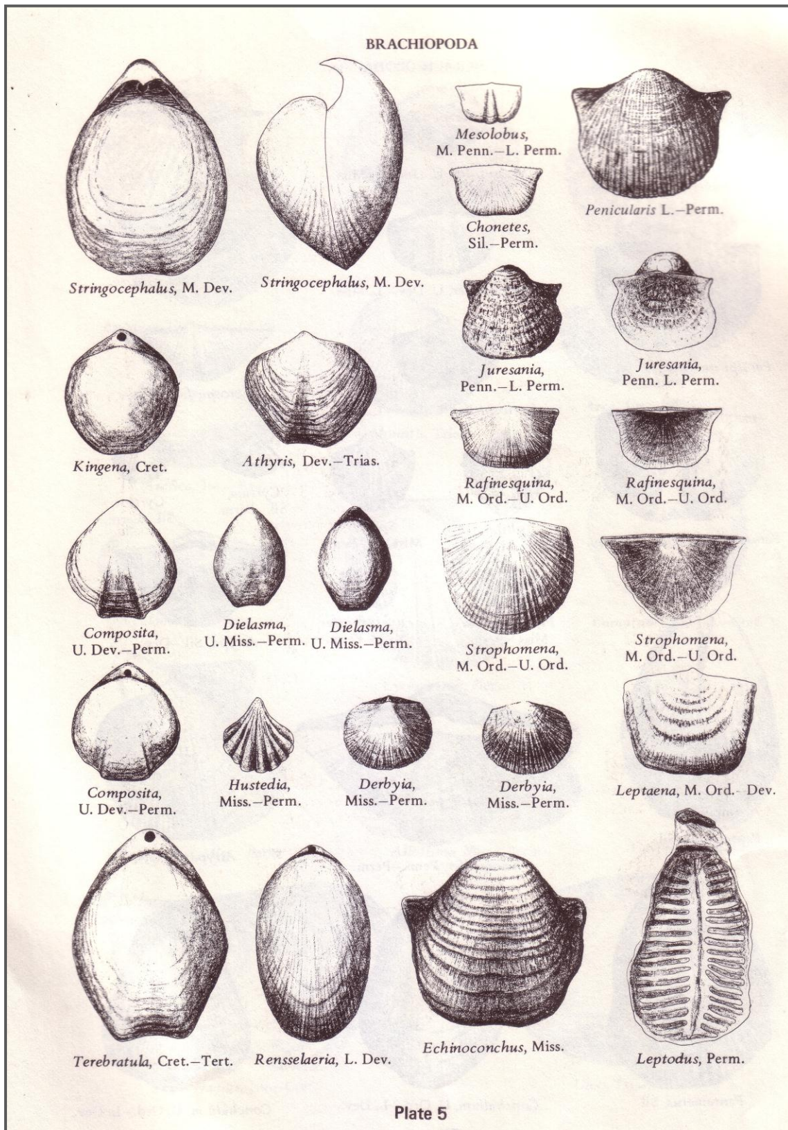
Gambar 3.20. Contoh Fossil Brachiopoda. Sumber : Interpreting earth history Morris s. petersen
